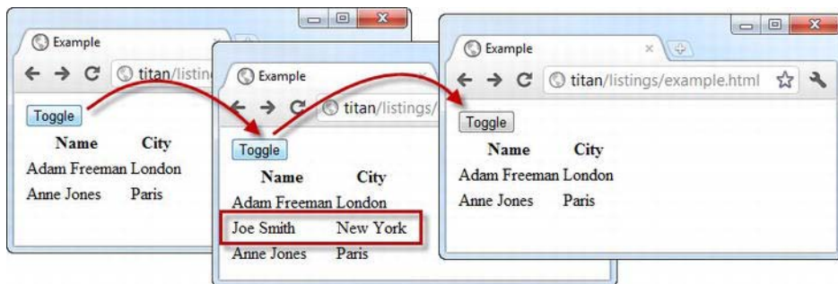
Figure 3-11. The effect of removing and adding the hidden element
