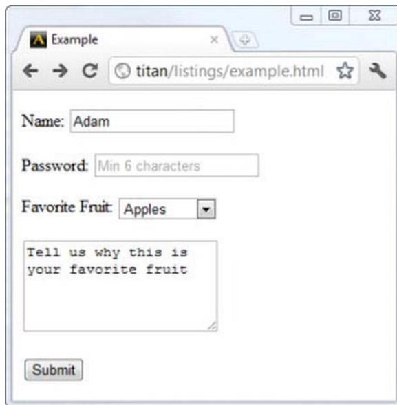
Figure 14-4. Using the textarea element
