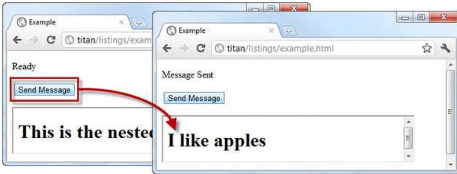
Figure 27-8. Using the cross-document messaging feature
