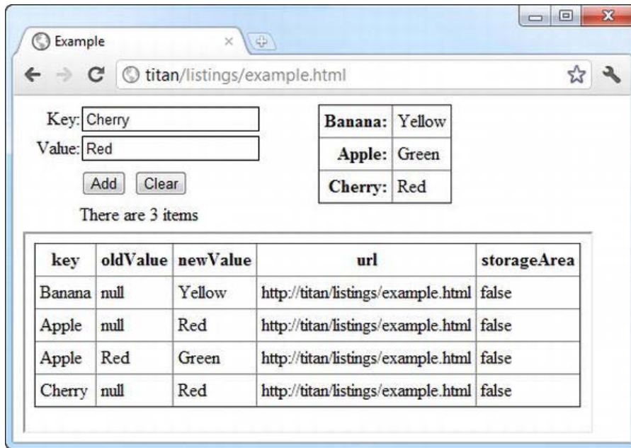
Figure 39-3. Storage events from session storage
