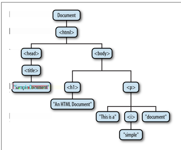
Figure 11-1. The tree representation of an HTML document
