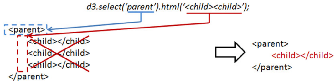
Figure 19-18. The html() operator replaces the contents of the parent tag with the tag passed as the argument
