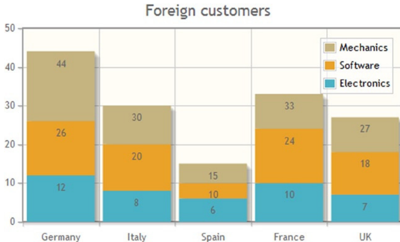
Figure 10-22. The default legend position is inside the chart, in the top-right corner
