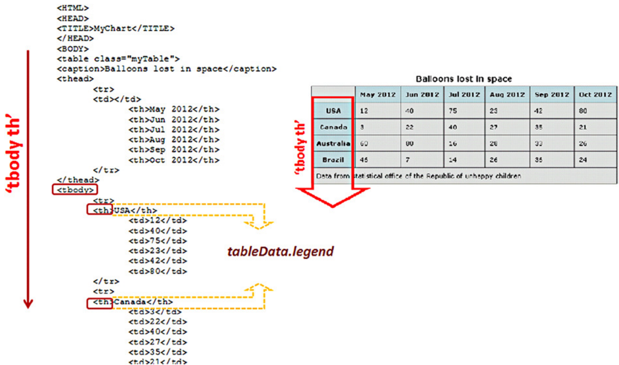
Figure 3-8. Parsing the names of countries with 'tbody th' as selector
