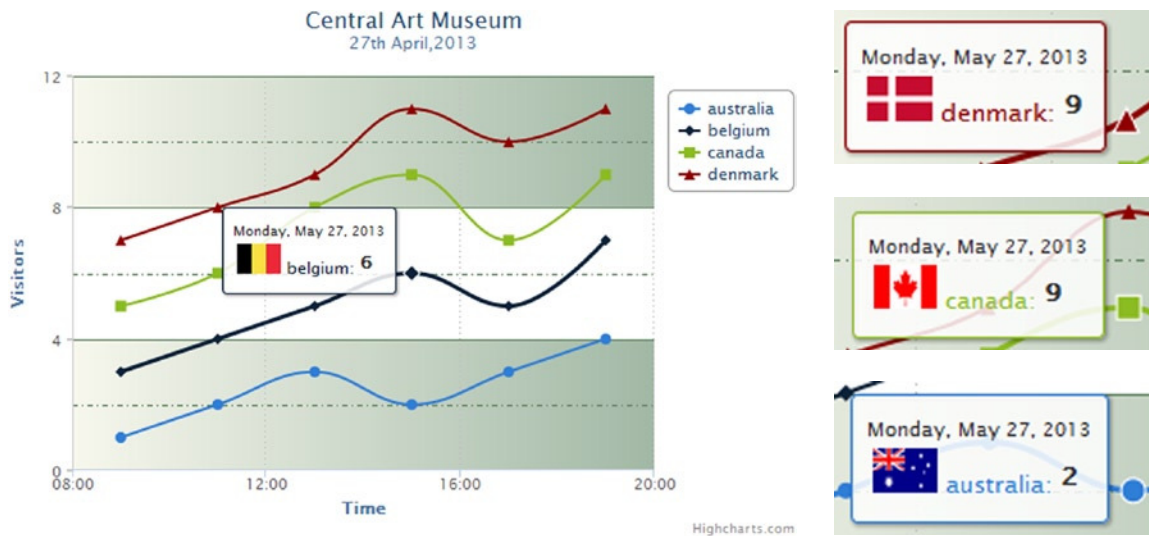
Figure 18-5. With the HTML customization of the tooltips, it is possible to modify their default layout
