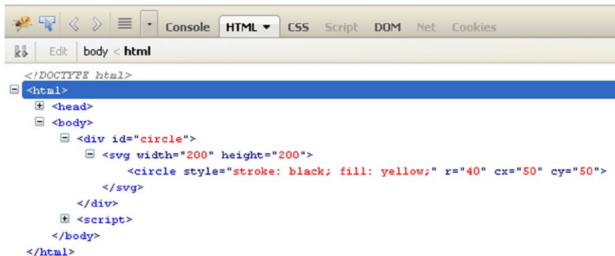
Figure 19-24. In FireBug, it is possible to follow the development of the tag structure
