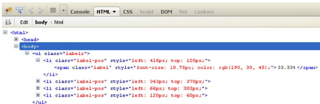
Figure 6-2. Using Firebug, it is possible to see the HTML structure dynamically generated
