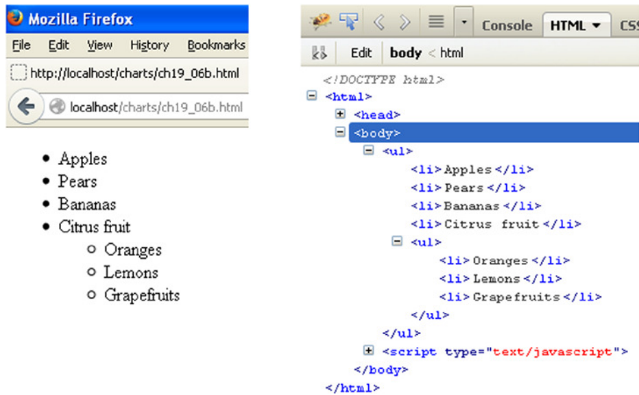
Figure 19-12. FireBug shows the HTML structure with a nested unordered list in the browser on the left and in FireBug on the right
