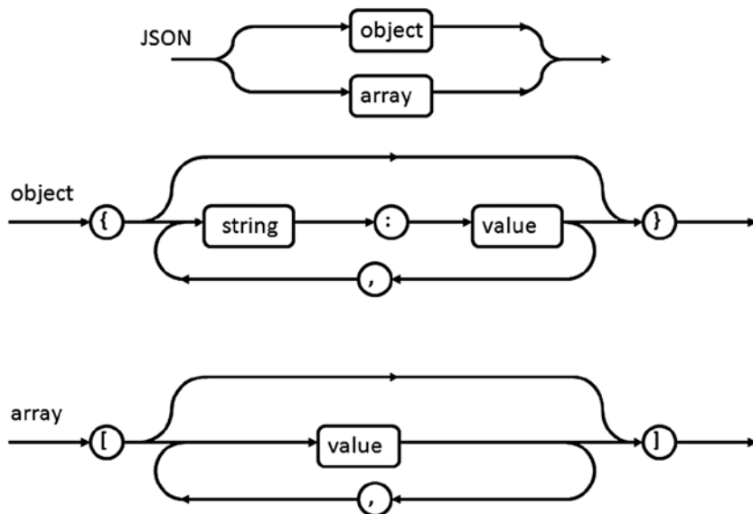
Figure 17-1. Syntax diagrams for JSON
