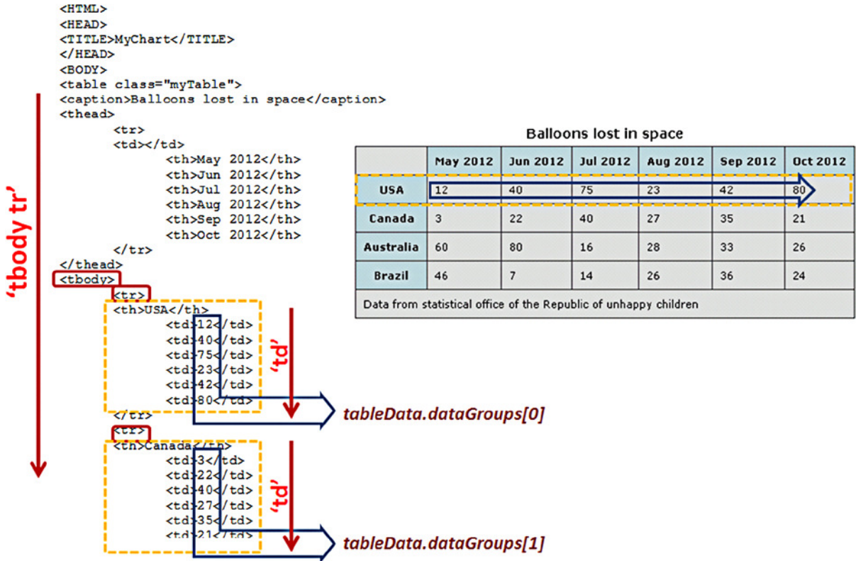
Figure 3-11. Parsing of groups of data for multiseries
