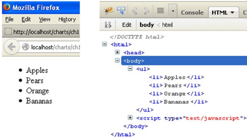
Figure 19-14. Using the CSS selector nth-child , you can add the Oranges item in any position in the list
