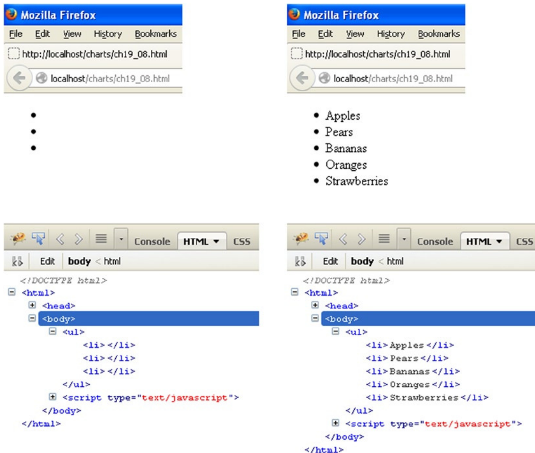
Figure 19-20. It is possible to fill the content of HTML elements with array values and to integrate them with other elements if they are not enough
