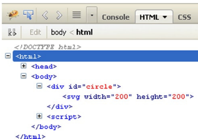
Figure 19-22. FireBug shows the <svg> tag you just created
