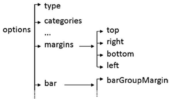
Figure 7-3. The hierarchy of the options object reflects the hierarchy of the elements that form the chart
