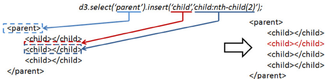
Figure 19-17. You can pass a child of the list as the argument using the CSS selector nth-child()
