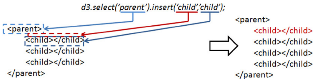
Figure 19-16. The insert() operator adds a child tag before the child tag is passed as a second argument
