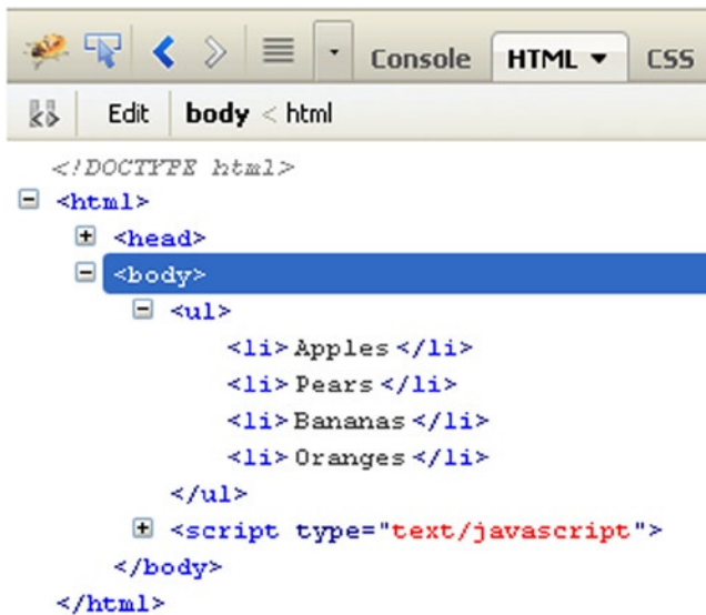
Figure 19-11. FireBug shows the HTML structure with the added <li> element
