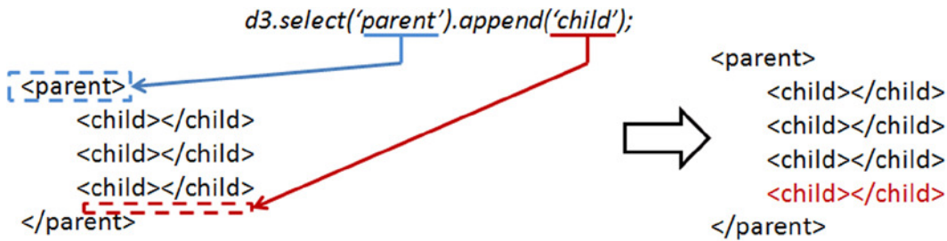
Figure 19-15. The append() operator adds a child tag to the end of the list
