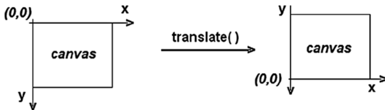
Figure 4-1. Canvas translation to obtain the origin point in the bottom-left corner
