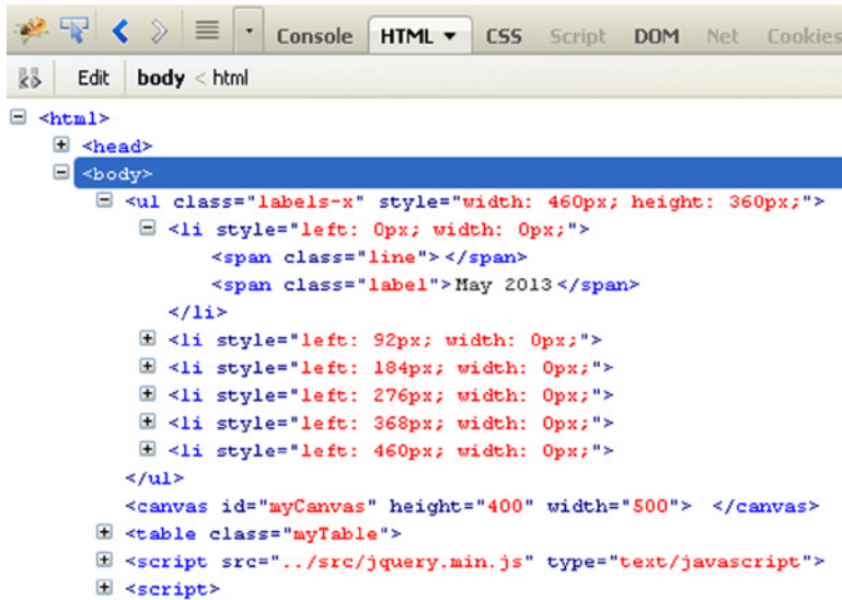
Figure 4-4. By selecting the HTML tab in Firebug, you can see the HTML structure dynamically generated
