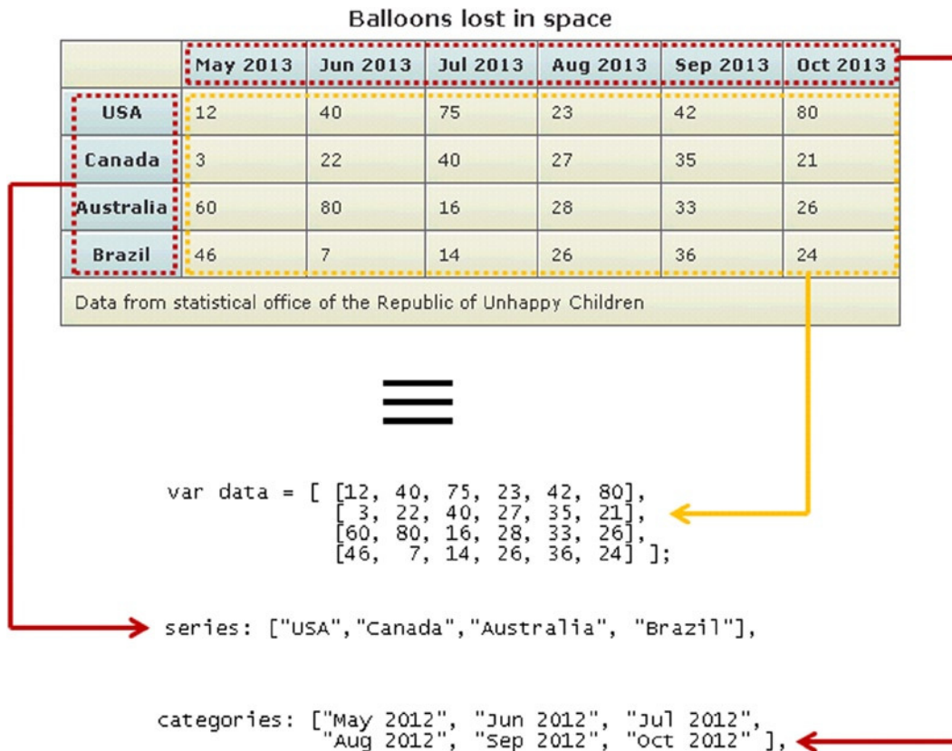
Figure 7-1. The input data can come from any kind of source (e.g., a table); the important thing to keep the data structure
